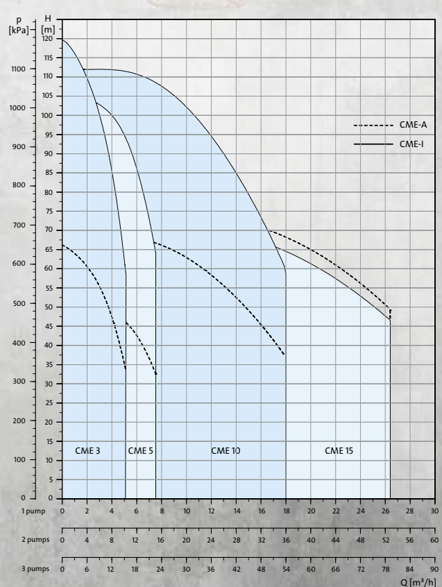
Performance curve: HYDRO MULTI-E, CME
