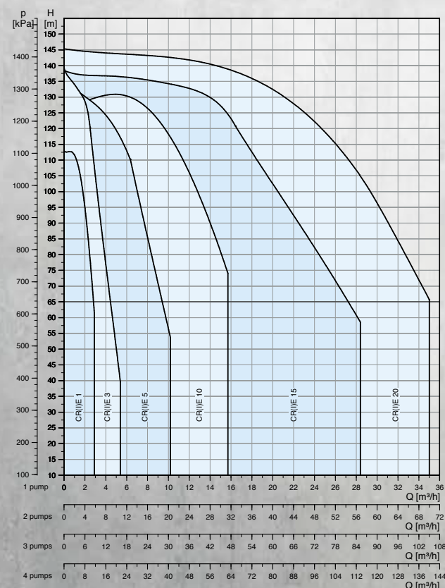
Performance curve: HYDRO MULTI-E, CRE/CRIE
